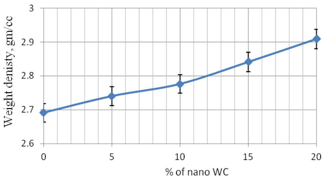
Fig 2: Effect of wt. % of Nano WC on density of Al/WC Nano MMCs
