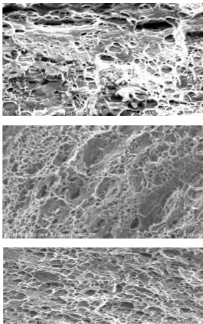
Fig. 7 (a) and (b) Fracture studies of Al/WC composites
